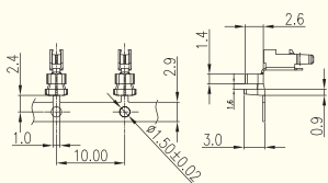
正向電源壓接母針 Load Side Power Crimp Socket XC-MC-6S-A1-4K (4000 pcs /Reel 卷)
